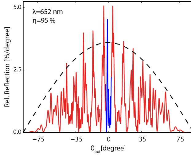
Figure 3 Broad-angle metasurface. Simulated angular scattering at \lambda=652 nm in the far field for the broad-angle metasurface illuminated at normal incidence composed of diffracted (red) and specularly reflected (blue) light. The dashed black line shows the angular profile of a perfect Lambertian diffusor.
