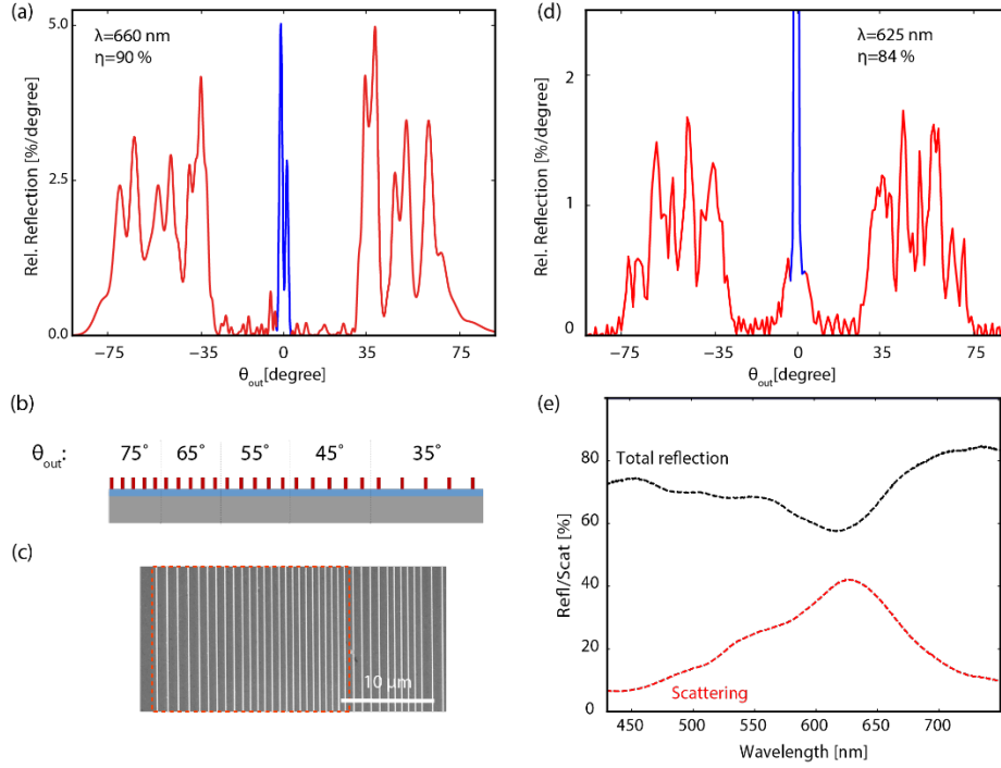
Figure 5 Large-angle reflector metasurface. (a) Numerical simulations of the angular reflection in far field for a single supercell of the large-angle reflector. (b) Schematic of the supercell. (c) SEM top view of the fabricated metasurface, the orange dashed box indicates a single supercell. (d) Angular reflection on resonance ( \lambda=625 nm). The red data indicate the diffracted scattering, the blue data specular reflection. (e) Total reflection (black) and scattering without specular reflection (red) of the large-angle reflector.
