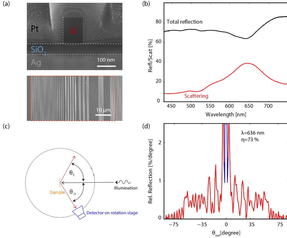
Figure 4 Fabricated broad-angle metasurface and optical measurements (a) top: Cross-section SEM image of a silicon bar on a \text{SiO}_x layer on Ag. To create image contrast the sample was covered with platinum before performing the FIB cross-section. Bottom: Top-view SEM image. The red dashed box represents a supercell composed of 7 differently pitched metagratings. (b) Total reflection (black) and scattering excluding specular reflection (red). (c) Schematic of angular scattering setup. The sample in the center of a rotating stage is illuminated with a vertical tilt of 10^\circ by a collimated p-polarized light beam (spectral bandwidth 2.5-5 nm). The detector on the rotating stage with a vertical tilt of -10^\circ collects the reflected power at a given horizontal angle \theta_{\text{out}} . (d) Measured angular reflection on resonance ( \lambda=636 nm). The red data indicate the diffracted scattering, the blue data specular reflection.
