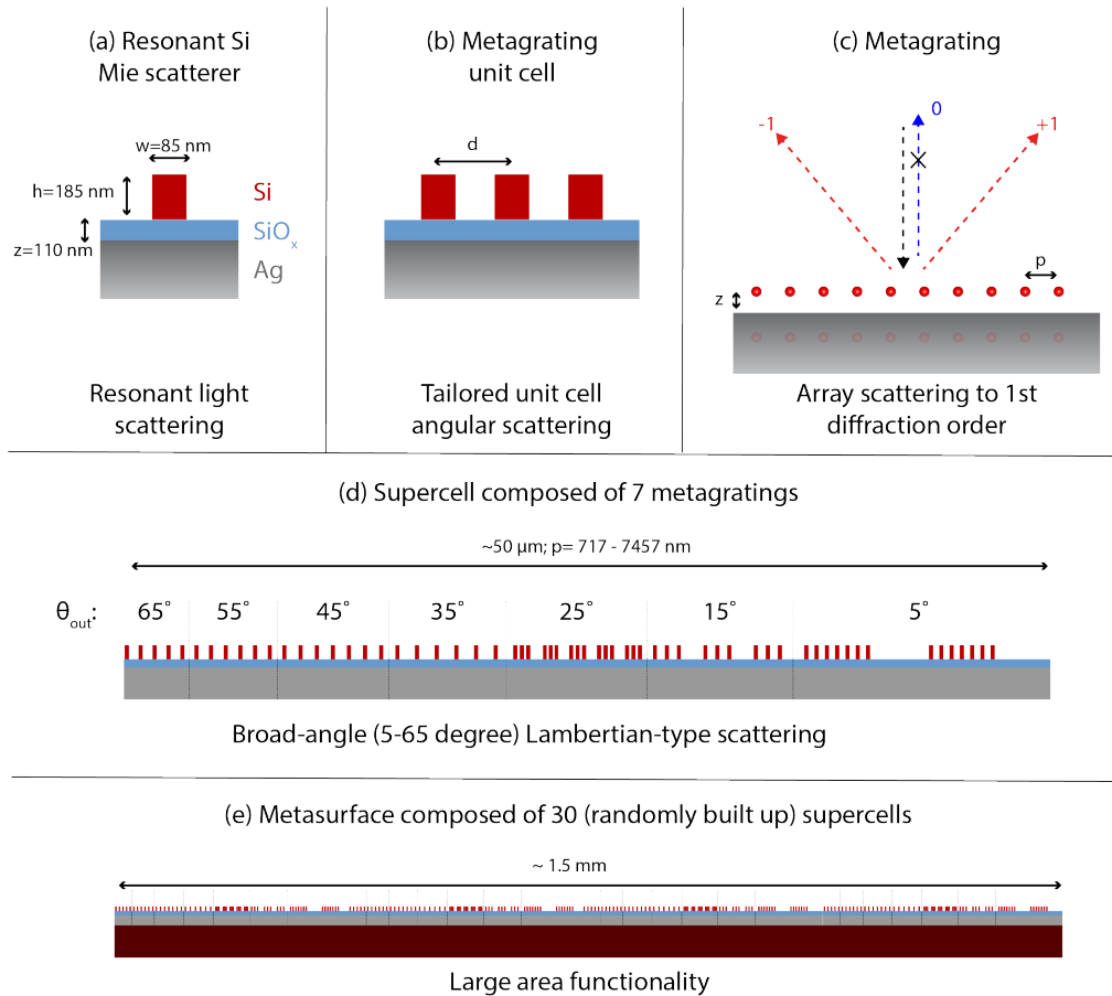
Figure 1 Metasurface design and length scales. Unit cells composed of one or more Si Mie resonators are arranged in a periodic array placed above a metal back plane to form a metagrating that scatters into only the \pm 1 diffraction orders. A supercell of metagratings creates a tailored angular response, and an array of supercells forms the large-area macroscopic metasurface.
