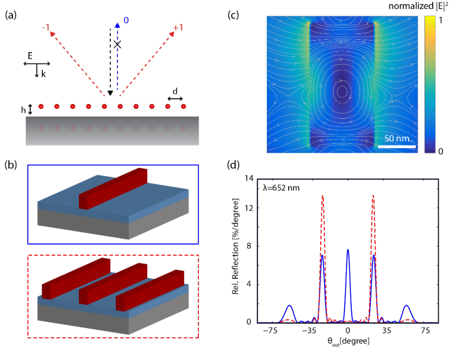
Figure 2 Magnetic dipole resonances in a 1D metagrating array (a) Periodic array of magnetic dipoles arranged over a ground plane. (b) Schematic of unit cells with one or three silicon bars on a silica spacer layer on top of a silver mirror. (c) Normalized electric field intensity |E|^2 and electric field lines (grey) in vertical crosscuts through an 85 nm wide and 180 nm tall Si bar on 110 nm \text{SiO}_x spacer layer on top of a silver mirror, parallel to the electric driving field. (d) Simulated angular scattering at \lambda=652 nm in the far field for a finite metagrating with just 5 periods with pitch of 1538 nm. Unit cells are composed of a single silicon bar (solid blue line) or three silicon bars (spaced by 230 nm; dashed red line) placed above a Ag ground plane with a 110 nm silica spacer. Light coupling to the specular reflection and second order diffraction is suppressed for the three-particle unit cell.
