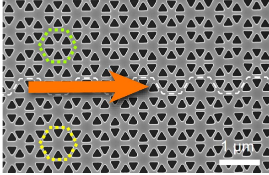
Fig. 1: Topological photonic crystal exhibiting the quantum spin Hall effect for light. The edge (white dashed line) separates two domains with differing bandstructure topology. The crystal structure is differentiated by the fact that the holes in the hexagonal unit cell are either closer together (green, 'shrunken lattice') or further apart (yellow, 'expanded lattice'). This deformation opens a bandgap on either side of the edge, which in turn supports a topological edge state.
