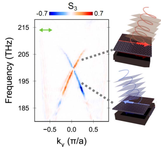
Fig. 2: Measured S_3 Stokes component of the reflected light vs frequency and in-plane wavevector, quantifying the degree of circular polarization in the output field. One recognizes that only the edge states in the photonic bandgap (between 190 and 208 THz) display pronounced circular polarization, whose helicity is linked to propagation direction (i.e., the group velocity of the states' dispersion curves). This reflects the photonic spin-orbit coupling that is responsible for the emergence of these quantum spin Hall-like edge states. Figure adapted from [8].
