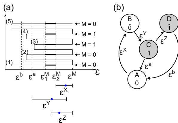
FIG. 5. (a) Scenario for the switching on and off of the modifying state M . The value of M in the range \epsilon_1^M < \epsilon < \epsilon_2^M (bold) is indicated for upsweep (1)-(5). (b) Tentative state diagram for additional degrees of freedom beyond hysteron 1-3. The system starts out in state A, and only after a sequence of up, down and up transitions, the system can reach the modifying state D, which leads to changes in the switching fields of hysterons 1 and 2.
