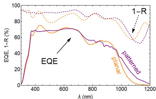
Figure 5. External quantum efficiency ( EQE ) and reflection losses ( 1-R ) of a fabricated planar (orange) and patterned (purple) PbS QD solar cell, as a function of wavelength. Solid lines describe EQE curves and dashed lines correspond to the upper limits for the EQE , given by the cell reflection and represented by 1-R .
