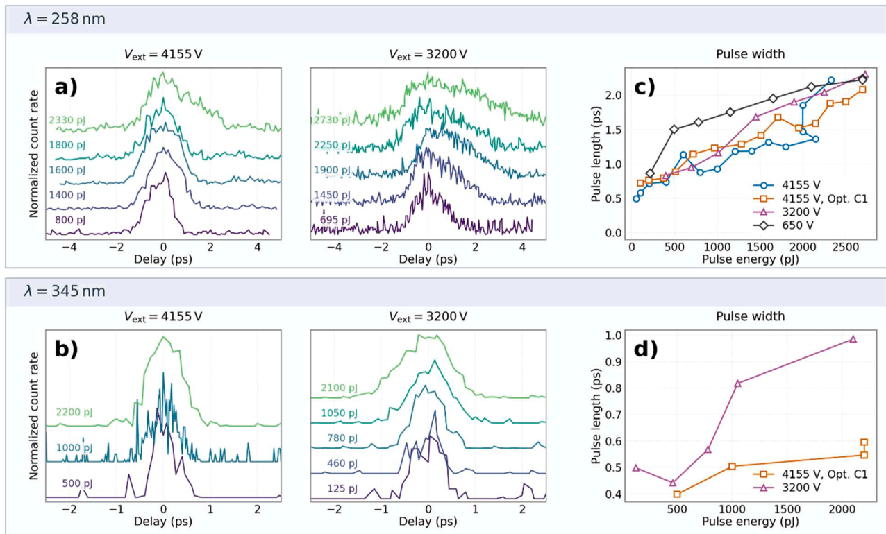
Fig. 4. Electron-light cross correlation measurements using light-electron coupling within dielectric laser accelerator structures. (a, b) Normalized count rate of electrons that gained energy as a function of relative delay between the electron and laser pulses at emitter excitation wavelengths (a) 258 nm and (b) 345 nm. (c,d) Extracted electron bunch lengths (2x RMS) after deconvolution of the 300 fs laser pulse that drives the DLA, for excitation at (c) 258 nm and (d) 345 nm.
