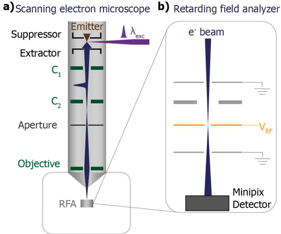
Fig. 1. (a) Schematic of the USEM setup. A fs laser beam excites a Schottky emitter to generate electron pulses. The electron beam goes through a set of lenses and is focused onto the retardation field analyzer (RFA), which is placed in the sample plane. (b) Schematic of the RFA setup. The electron beam is focused onto the retarding electrode, the retarding voltage V_{\text{RF}} is then scanned around the voltage of the beam while the transmitted electrons are detected downstream by the Minipix detector.
