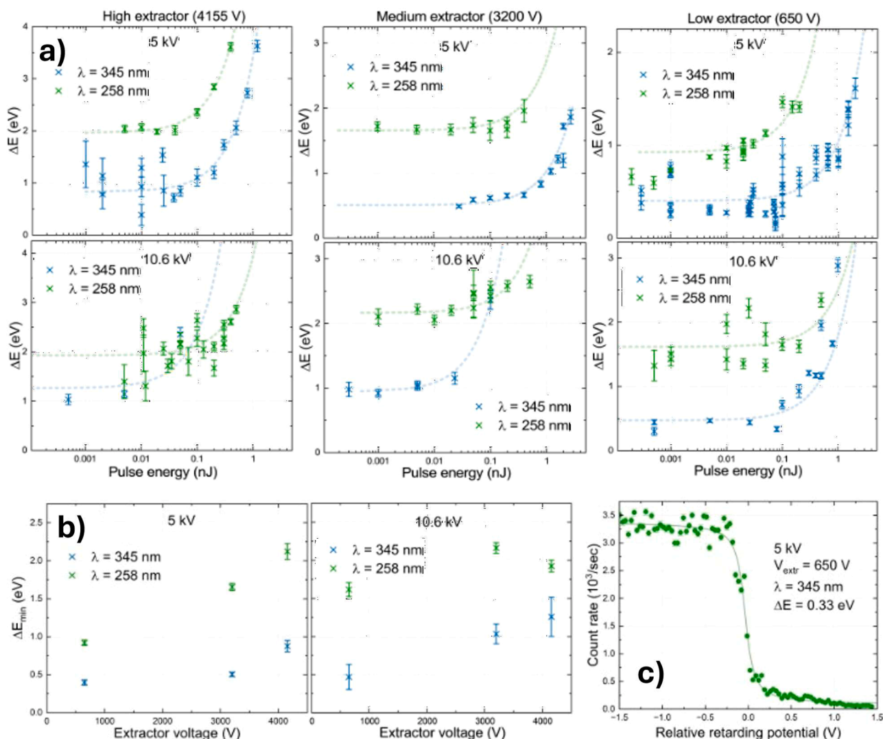
Fig. 3. Overview of the electron beam energy width (FWHM) measurements. Panel (a) shows energy width (FWHM) based on laser pulse energy, wavelength and gun voltage settings. All fits are linear functions. At low laser powers, 345 nm excitation consistently gets better energy resolution than excitation at 258 nm, while same applies for low extractor regime compared to medium and high extractor regimes across the board. The limits of energy widths from fits (i.e. intercepts of fit with pulse energy = 0 axis) are plotted in panel (b). Panel (c) shows an example of RFA type measurement fitted with cumulative distribution function of Pseudo-Voigt distribution.
