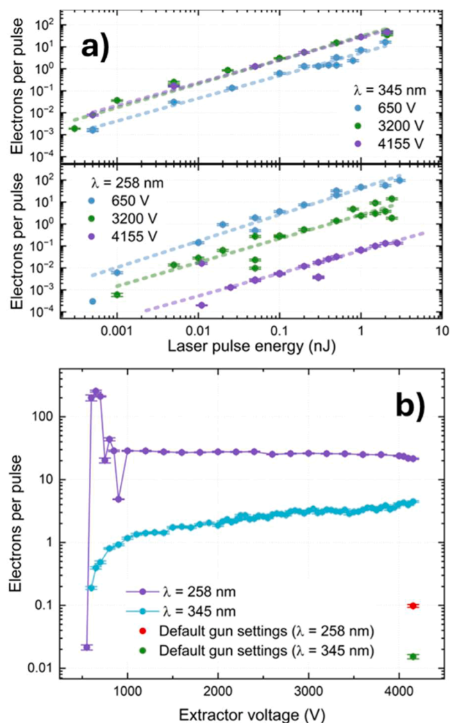
Fig. 2. Number of electrons generated per pulse at various settings. (a) Dependence on laser pulse energy while driven with 345 nm wavelength and 258 nm. Overall the current scales linearly with pulse energy at all extractor settings. (b) Dependence on extractor voltage for constant laser power. The red and green data point are for the default gun spot setting without optimization by the C1 lens voltage.
