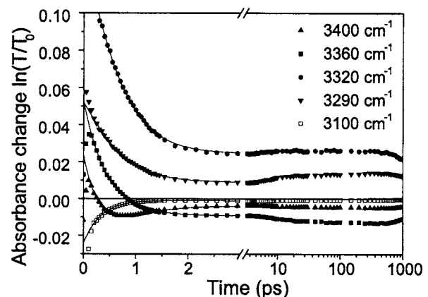
FIG. 5. Pump induced absorbance change plotted as a function of probe delay at various probe frequencies. From 3 ps onwards absorbance changes are observed related to slow collective rearrangements of the hydrogen bonded crystal lattice.
