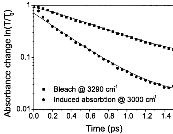
FIG. 3. Pump induced absorbance change plotted as a function of probe delay at 3290\text{ cm}^{-1} (center frequency bleaching) and 3000\text{ cm}^{-1} (center frequency induced absorption). Both curves are scaled to equal amplitude and sign to facilitate comparison of the dynamics. The relaxation is faster for the induced absorption than for the bleaching.
