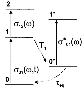
FIG. 4. Schematic overview of the model that describes the population dynamics of excited HDO molecules. Relaxation from the excited \nu_{\text{OH}}=1 state proceeds via an intermediate level 0^* with associated OH-stretch cross section \sigma_{01^*}^*(\omega) that is different from the cross section \sigma_{01}^*(\omega, t) in the ground state.
