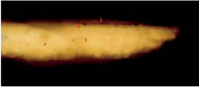
Fig. 9 Cross-section of ground and imprimatura of The Death of Achilles (without drawing and paint) normal light dark field, taken at 200x magnification . Layer 3: Old varnish Layer 2: Imprimatura with black charcoal particles Layer 1: Chalk/glue ground
