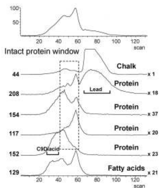
Fig. 15 DTMS data on the imprimatura from panel 13 showing the total ion current trace and mass chromatograms of ions from chalk (m/z 44), intact proteins (m/z 152, 117, 154, 208) and a general marker for saturated fatty acids (m/z 129). Note the appearance of lead (m/z 208) in scan window 60-100. The degraded proteins appear in a higher temperature window compared to the ground. M/z 152 appears as a broad peak and includes the marker for azelaic acid (C9 diacid) between scan 20-40
