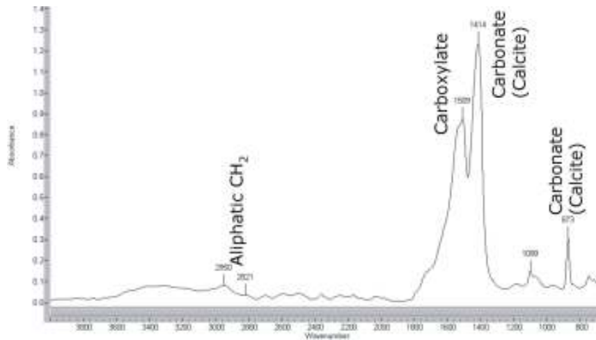
Fig. 16 FTIR transmission spectrum of the imprimatura layer from 1760 e showing chalk (calcite), lead carboxylate, and the absence of lead white (no peak at 680 cm -1 )
