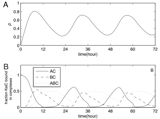
Fig. 3. Sustained oscillations in the full model defined by Eqs. 6–10. (A) The mean phosphorylation level p of KaiC shows a stable 24-h rhythm. (B) Kai complexes. At t = 0 , KaiC is fully unphosphorylated: [C_0] = [C]_T ; [A] = [A]_T ; [B] = [B]_T . The average phosphorylation then increases as KaiA binds KaiC and stimulates phosphorylation. Next, the amount of KaiB–KaiC complex ([BC]) increases at high phosphorylation as KaiB binds to the inactive state of KaiC. Subsequently, KaiA is sequestered into a KaiA–KaiB–KaiC complex (ABC). The total concentrations equal those used in the in vitro experiments described in ref. 3: [C]_T = 0.58 \mu\text{M} ; [A]_T = 1.75 \mu\text{M} ; [B]_T = 0.58 \mu\text{M} , corresponding to [A]_T = [C]_T and [B]_T = 3[C]_T . For other parameter values, see Table 2 of SI Appendix .
