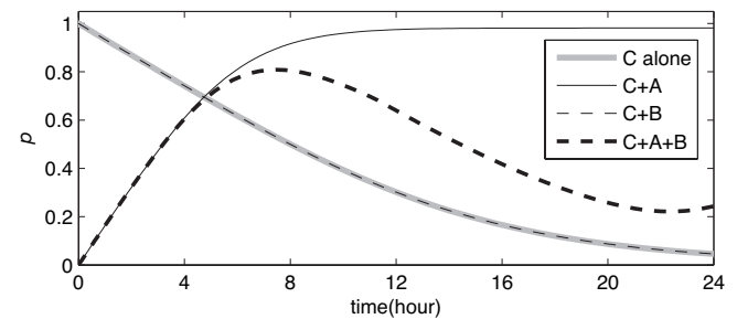
Fig. 4. KaiC phosphorylation in the absence of KaiA and KaiB (C alone), in the presence of KaiA (C+A), in the presence of KaiB (C+B), and in the presence of both KaiA and KaiB (C+A+B). For C+A, KaiC is initially fully unphosphorylated; for C alone and C+B, KaiC is initially fully phosphorylated (see also ref. 7). Parameters are as in Fig. 3.
