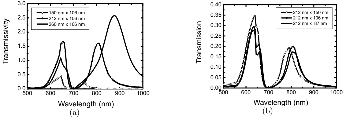
FIG. 10: Calculated transmissivity spectra for y -polarized incident light of arrays in a Au film in which the shape of the holes is varied by increasing only on side of the rectangles. (a) hole side along y -direction constant. (b) hole side along x -direction constant.
