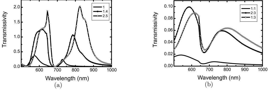
FIG. 9: Calculated transmissivity spectra for y -polarized light and for rectangular hole arrays with different aspect ratio. (a) Transmissivity through arrays in a Ag film. (b) Transmissivity through arrays in a Ni film.
