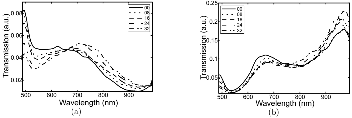
FIG. 6: (a) The normalized spectra for the random square hole is plotted for different angles of incidence. (b) The normalized spectra for random rectangle (aspect ratio 3) hole arrays are shown. The wavelengths of the maxima and minima stay almost at the same positions. Only for the squares a small shift can be seen of the peak around 700 nm, a shift that is 8 times smaller than we measured for periodic hole arrays. In the legend the angle of incidence is listed.
