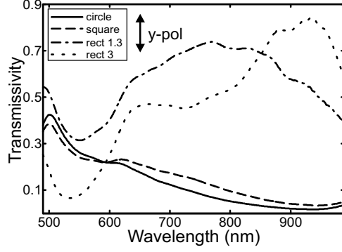
FIG. 5: The transmissivity of random hole arrays in Au for three forms: circles with a diameter of 190 nm, squares ( 170 \times 170 \text{ nm}^2 ) and two types of rectangles with an aspect ratio of 2:3 ( 150 \times 225 \text{ nm}^2 ) and of 1:3 ( 75 \times 225 \text{ nm}^2 ). For increasing aspect ratio, the position of the peak shifts to longer wavelengths and the transmissivity increases.
