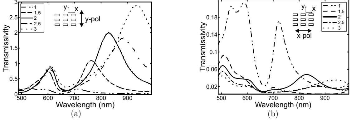
FIG. 2: The transmissivity of structures with different aspect ratio of the holes while keeping the hole area constant for two different polarizations of light. The legends show the aspect ratios of the holes. In the insets the used axes are displayed. (a) The transmissivity for y-polarized light shows an increase in transmissivity by an increase in aspect ratio. The peaks are broadened and shift to longer wavelengths. (b) For x-polarized light the opposite occurs: a decrease in aspect ratio leads to an increase in transmissivity.
