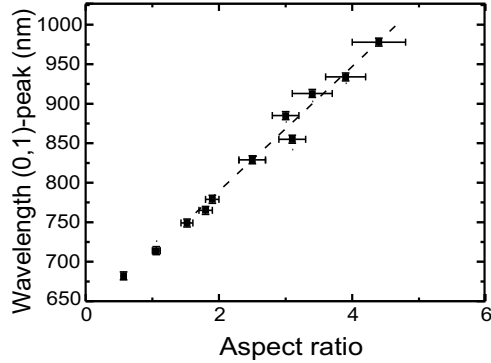
FIG. 3: The wavelength of the (0,1)-peak as function of aspect ratio. The peak shifts monotonously to longer wavelengths when the aspect ratio increases.
