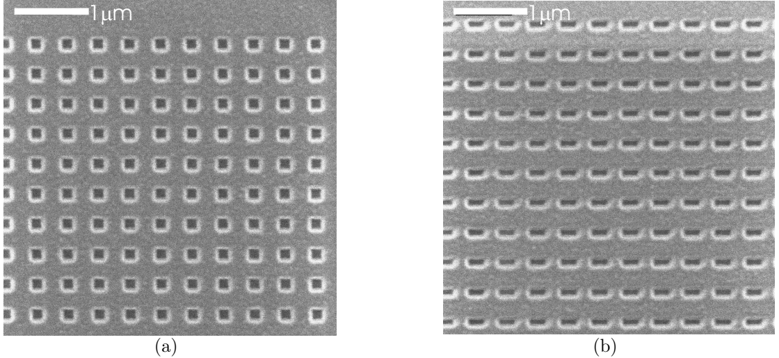
FIG. 1: Focused ion beam images of two periodic arrays: (a) square holes with an aspect ratio of 1 (size: 150 \times 150 \text{ nm}^2 ) and (b) rectangular holes with an aspect ratio of 2 (size: 106 \times 212 \text{ nm}^2 ). Both structures are fabricated in a 200 nm thin Au layer and have a periodicity of 425 nm. The holes have sharp edges and are highly uniform.
