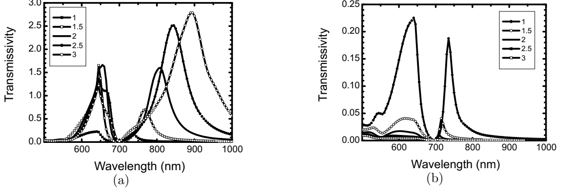
FIG. 8: Calculated transmissivity spectra for periodic hole arrays in a Au film with different aspect ratio (the surface area of the hole and the thickness are constant and identical to those used in the experiments). (a) transmissivity for y-polarized light. (b) transmissivity for x-polarized light
