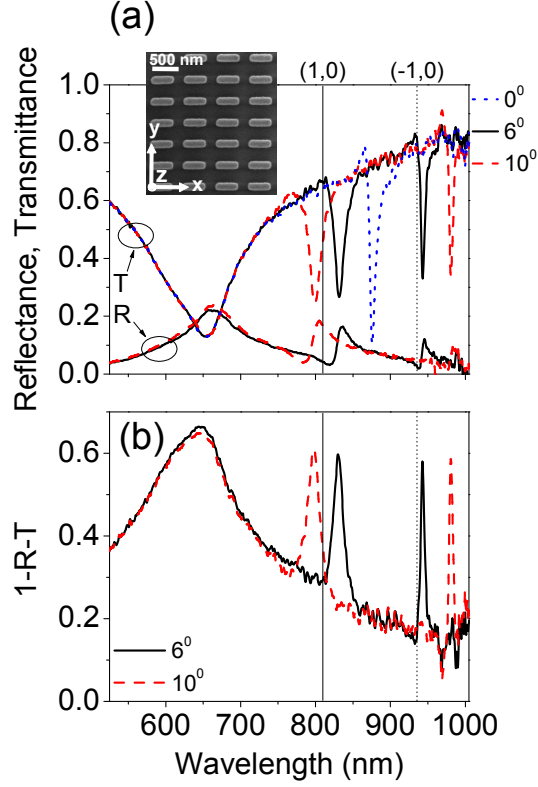
FIG. 1: (Color online). (a) Zero-order transmittance, T , through and specular reflectance, R , from a plasmonic crystal of nanoantennas as a function of wavelength for different angles of incidence, \theta = 6^\circ (black solid lines), \theta = 10^\circ (red dashed lines), respectively. Transmittance at normal incidence is shown by the blue dotted line. Light is polarized along the y direction. The wave vector component of the incident wave parallel to the array surface is along the x direction. The vertical solid and dotted lines indicate the (1,0) and (-1,0) Rayleigh anomalies at 6^\circ , respectively. Inset: scanning electron microscope image of a plasmonic crystal of nanoantennas. (b) 1 - R - T as a function of wavelength for 6^\circ (black solid line), 10^\circ (red dashed line).
