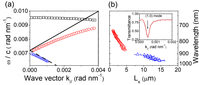
FIG. 3: (Color online). (a) Experimental dispersion relations of the (1,0) and (-1,0) lattice surface modes (red circles and blue triangles, respectively), and of the localized surface plasmon resonance (black squares). The normalized frequency \omega/c is plotted versus the parallel wave vector k_{||} . The Rayleigh anomaly associated to the (1,0) and (-1,0) diffraction orders in amorphous quartz is represented by the solid and dashed lines, respectively. (b) Propagation length L_x as a function of wavelength for the (1,0) and (-1,0) lattice surface modes (red circles and blue triangles, respectively). Inset: Transmittance spectrum (red line) and its Lorentzian fit (black dotted line) as a function of k_{||} at \omega/c = 0.00738 \text{rad nm}^{-1} ( \lambda = 851 nm).
