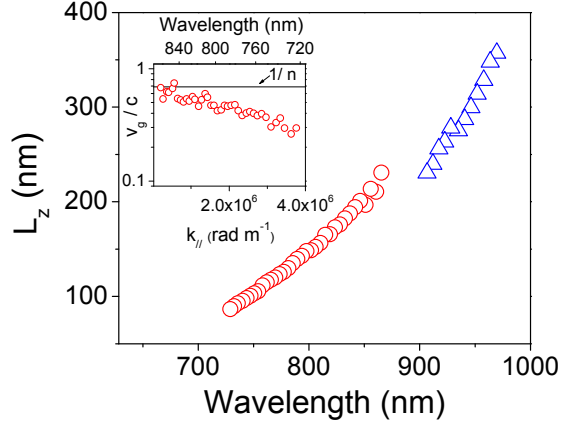
FIG. 4: (Color online). Decay length L_z as a function of wavelength for the (1,0) (red circles) and (-1,0) lattice surface modes (blue triangles). Inset: Group velocity normalized to speed of light in vacuum associated to the (1,0) mode as a function of the wave vector k_{\parallel} and wavelength. The horizontal line indicates the normalized speed of light in amorphous quartz ( n = 1.45 ).
