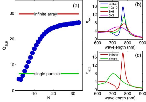
Figure 3: (a) Calculated quality factor of SLRs ( Q_{SLR} ) as a function of the number of particles ( N ) along each dimension of the array. (b) Calculated extinction spectra for some of the arrays yielding the increasing Q_{SLR} in (a). (c) Calculated extinction spectra of a single particle and an infinite array. The quality factors of the single particle and the infinite array are indicated by the horizontal lines in (a).
