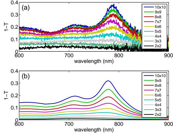
Figure 1: (a)Measurements, (b) Coupled Dipole Model calculations, of the extinction spectra of N \times N gold nanodisk arrays, where N ranges from 2 to 10.
