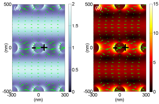
Figure 4: Total field enhancement (color scales) and scattered field (arrows) for an infinite array of gold nanodisks surrounded by amorphous quartz. Both plots are at a plane intersecting the nanodisks at their midheight. The illumination is a normally incident plane wave with a vacuum wavelength of (a) \lambda = 670 nm, and (b) \lambda = 780 nm, which correspond to the wavelengths of the LSPR and SLR, respectively. The polarization vector is along the same axis as the excited dipole moment in the individual particles, indicated by the + and - signs.
