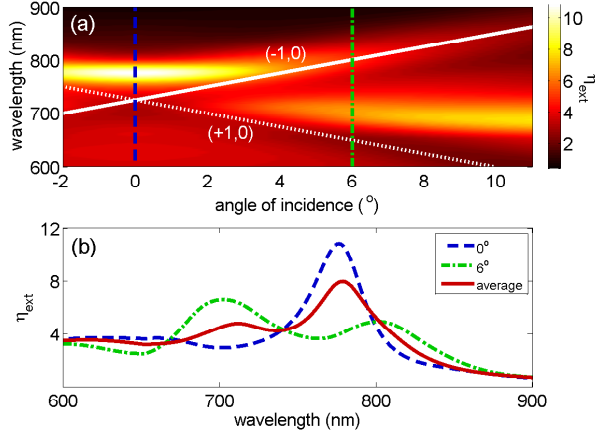
Figure 2: Coupled Dipole Model calculations for an array of 10x10 gold nanodisks. (a) Variable angle extinction spectra, (b) the dashed and dashed-dotted curves are cuts at \theta = 0^\circ and \theta = 6^\circ of (a), respectively, and the solid curve is the average extinction between 0 and 6 degrees.
