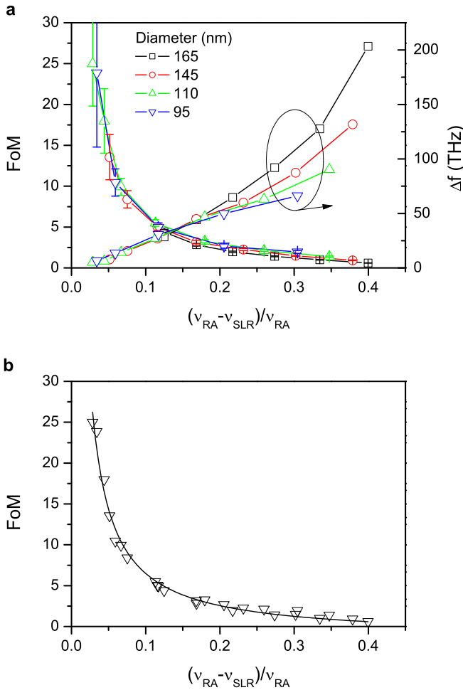
Figure 4: Measured FoM for different gold nanoparticle arrays and fit of the experimental data. a , Experimental FoM \frac{\partial \lambda / \partial n}{\Delta \lambda} and the full width at half maximum \Delta f of surface lattice resonances as a function of the detuning parameter (\nu_{RA} - \nu_{SLR})/\nu_{RA} for particle arrays with diameters 95, 110, 145, 165 nm, height 50 nm and lattice constant a = 300, 350, 400, 450, 500, 550 and 600 nm. b , Fit of the experimental data indicating a reciprocal scaling of the FoM with the detuning using y = 0.79/x - 1.38 .
