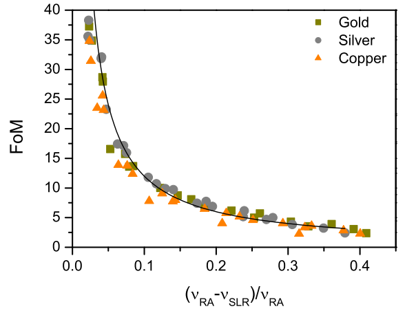
Figure 5: Calculated FoM for gold, silver and copper nanoparticle arrays. Calculated FoM for gold (squares), silver (dots) and copper (triangles) nanoparticle arrays with diameters 95, 110, 145, 165 nm, height 50 nm and lattice constant a = 300, 350, 400, 450, 500, 550 and 600 nm as function of (\nu_{RA} - \nu_{SLR})/\nu_{RA} . The solid line is a fit to the data using y = 1.2/x .
