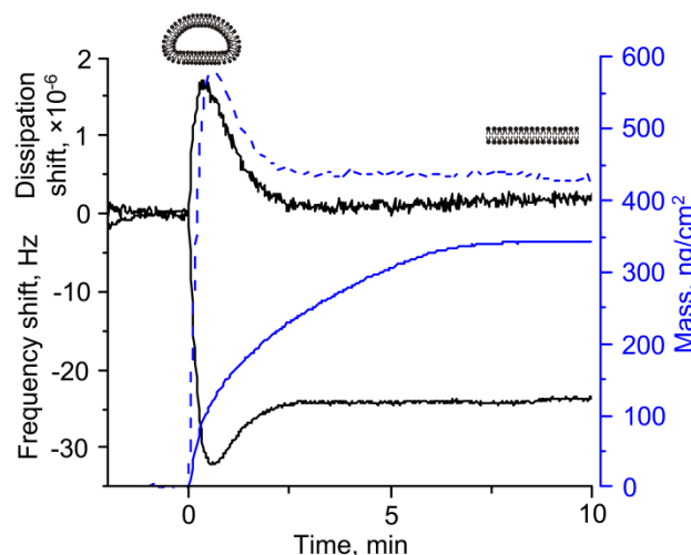
Figure 2: Bilayer formation from sonicated dioleoyl choline liposomes on silica is monitored by an optical (ellipsometry) and acoustic (quartz crystal microbalance) techniques. For QCM, the raw data (frequency and dissipation shifts, black solid lines) are plotted as well as the mass derived from the frequency shift using the Sauerbrey relationship 30 ( m = 18.1 \cdot \Delta f , where \Delta f is the frequency shift in Hz, dashed blue line). For ellipsometry, the optical mass is plotted directly (solid blue line). There is a very clear difference between the two responses. While QCM data contains the extrema in the signals (frequency and dissipation), first identified by Keller and Kasemo, 34 the optical response simply shows a continuous increase in the mass of the lipids present on the surface and is not able to distinguish between adsorbed liposomes and bilayers (diagrams shown above the curves). Note also that the final mass obtained by the two techniques is not the same. This could be due to the residual liposomes associated with the bilayer or imprecise assumptions used in the calculation of the optical mass from the raw ellipsometric data. For the QCM signals, the data on the 5th overtone, scaled by the overtone order, is plotted. Credits: The data was obtained with a combined QCM-D – Ellipsometry instrument based on the M2000 V spectroscopic ellipsometer from Woollam, Inc. (NE, U.S.A.) and Q-Sense E1 system (Biolin Scientific AB, Västra Frölunda, Sweden) equipped with an open module with a home-made trapezoidal glass cuvette clamped to it over the crystal. The data is a courtesy of Dr. Ralf Richter from CIC biomaGUNE (Spain) and the Max Planck Institute for Intelligent Systems, (Stuttgart, Germany).
