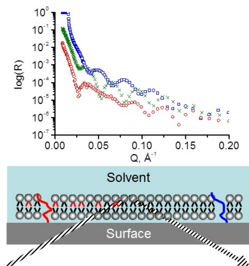
Figure 6: Schematic representation of a neutron reflectometry experiment. A neutron (grey dashed lines) beam goes through the substrate (silicon block) and is reflected from the substrate/lipid and lipid/solvent interfaces. The resulting reflectivity curves (above) are fitted with a model that yields the scattering length density (sld) distribution in the direction normal to the interface (red and blue overlays over the lipid molecules). In this case, on the left the bilayer is asymmetric while on the right it is symmetric. If one of the two lipids is deuterated (black) and the other one is not (red), this asymmetry can be detected (notice that the red and the blue sld profiles are different). The asymmetry may be caused by a number of factors (see references in the text): The “red” and the “black” lipids typically differ in some way – e.g., headgroup, or chain length/composition. Deuteration is not the cause of the asymmetry but merely enables its detection. The sld profiles, as well as the reflectivity data, shown in this figure are from an actual experiment where lipid distribution on TiO 2 was studied (Figure credit: Reviakine et al. KIT).
