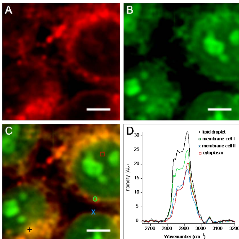
Figure 4: Hyperspectral image plots of HCT116 (colorectal carcinoma) cells after 12h of culture from Multiplex CARS microscopy. (A) Intensity map primarily showing CH 2 symmetric vibrations [2840-2846 cm -1 ], which allows label-free identification of cell membranes and lipid droplets. (B) Intensity map showing CH 3 vibrations [2900-2930 cm -1 ], which is indicative of protein organization. (C) Overlay of A and B clearly shows cellular structures containing only protein (green) or lipids (red) are identifiable from label-free microspectroscopy. Inspection of the overlay demonstrates the appearance of condensed protein, possibly chromatin masses, that do not colocalize with membrane structures. (D) Raman spectra from different voxels in C provide quantitative information on the respective lipid composition and lipid-protein ratio. Scale bar = 5 μm. Image courtesy of N. Billecke, W. Gebhardt, and S. H. Parekh (Max Planck Institute for Polymer Research).
