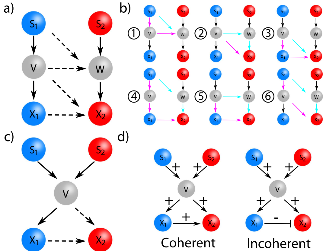
Figure 1. Overview of networks. Each network consists of two pathways S1 \rightarrow X1 (Left) and S2 \rightarrow X2 (Right). The pathways may interact via regulatory interactions and a shared component. Solid arrows are either activating or repressive, while dashed arrows can be activating, repressive or absent. a ) 6 node topology. b ) 6 different possible incoherent feed-forward loops marked by colored arrows (magenta activating, light blue repressing) c ) 5 node topology. d ) example of an incoherent and coherent feed-forward loop for a 5 node topology (+ activating, – repressing).
