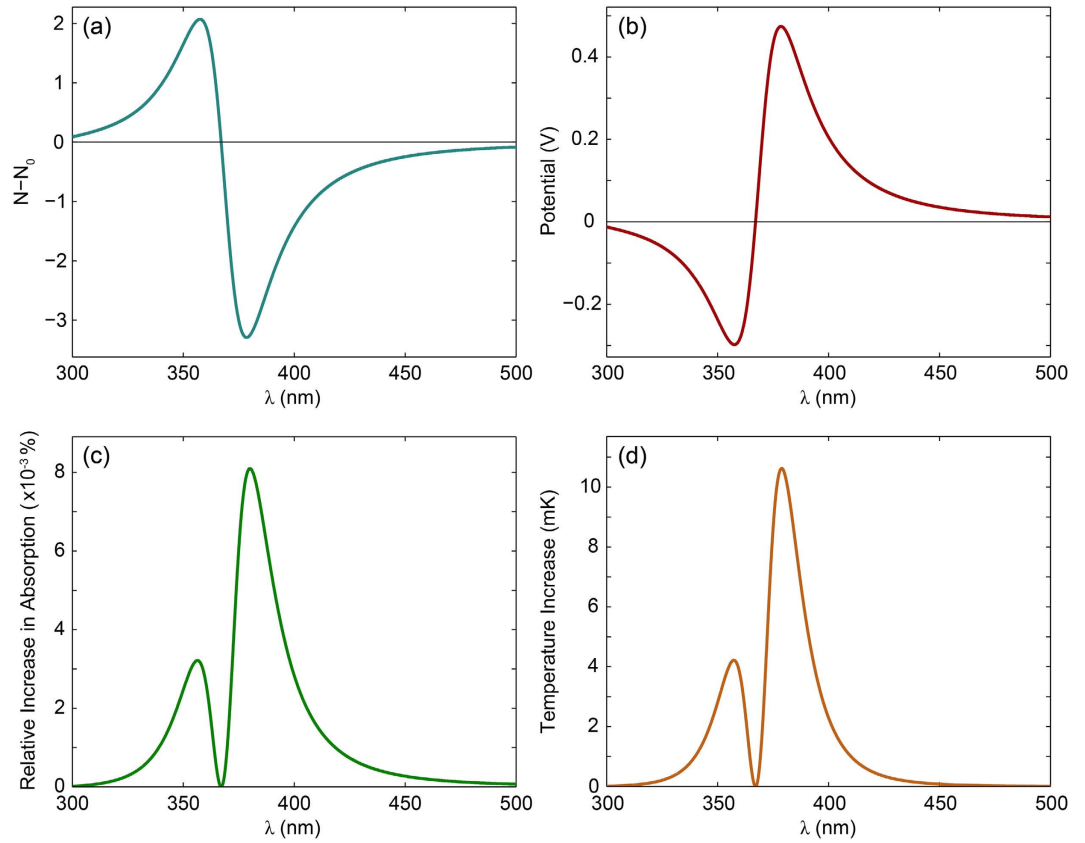
Figure 4. Steady-state configuration as a function of wavelength of a 20 nm Ag particle in vacuum under I_\lambda = 100 \text{ W/m}^2 monochromatic illumination. (a) Time-averaged number of electrons transferred from the substrate into the nanoparticle. (b) Induced plasmoelectric surface potential. (c) Relative increase in absorption as result of plasmoelectric effect. (d) Corresponding increase in particle temperature compared with a particle that remains neutral.
