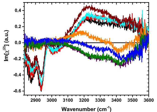
Fig. 2 Imaginary \chi^{(2)} spectra of aqueous PAA at different pH and corresponding different degrees of ionization \alpha : pH = 2.8 ( \alpha \approx 0.046 ) [black], pH = 3.3 ( \alpha \approx 0.068 ) [red], pH = 4.2 ( \alpha \approx 0.134 ) [cyan], pH = 4.8 ( \alpha \approx 0.203 ) [brown], pH = 5.3 ( \alpha \approx 0.278 ) [orange], pH = 6.1 ( \alpha \approx 0.428 ) [purple], pH = 12.6 ( \alpha \approx 1 ) [green] and water [blue].
