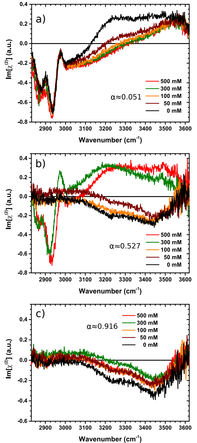
Fig. 3 Spectra of PAA (4.5 g/L) with different NaCl concentrations added: 0 mM NaCl (black), 50 mM NaCl (brown), 100 mM NaCl (yellow), 300 mM NaCl (green), 500 mM NaCl (red). The values for \alpha are calculated via equation(1) and correspond to the solutions with 0 mM NaCl.
