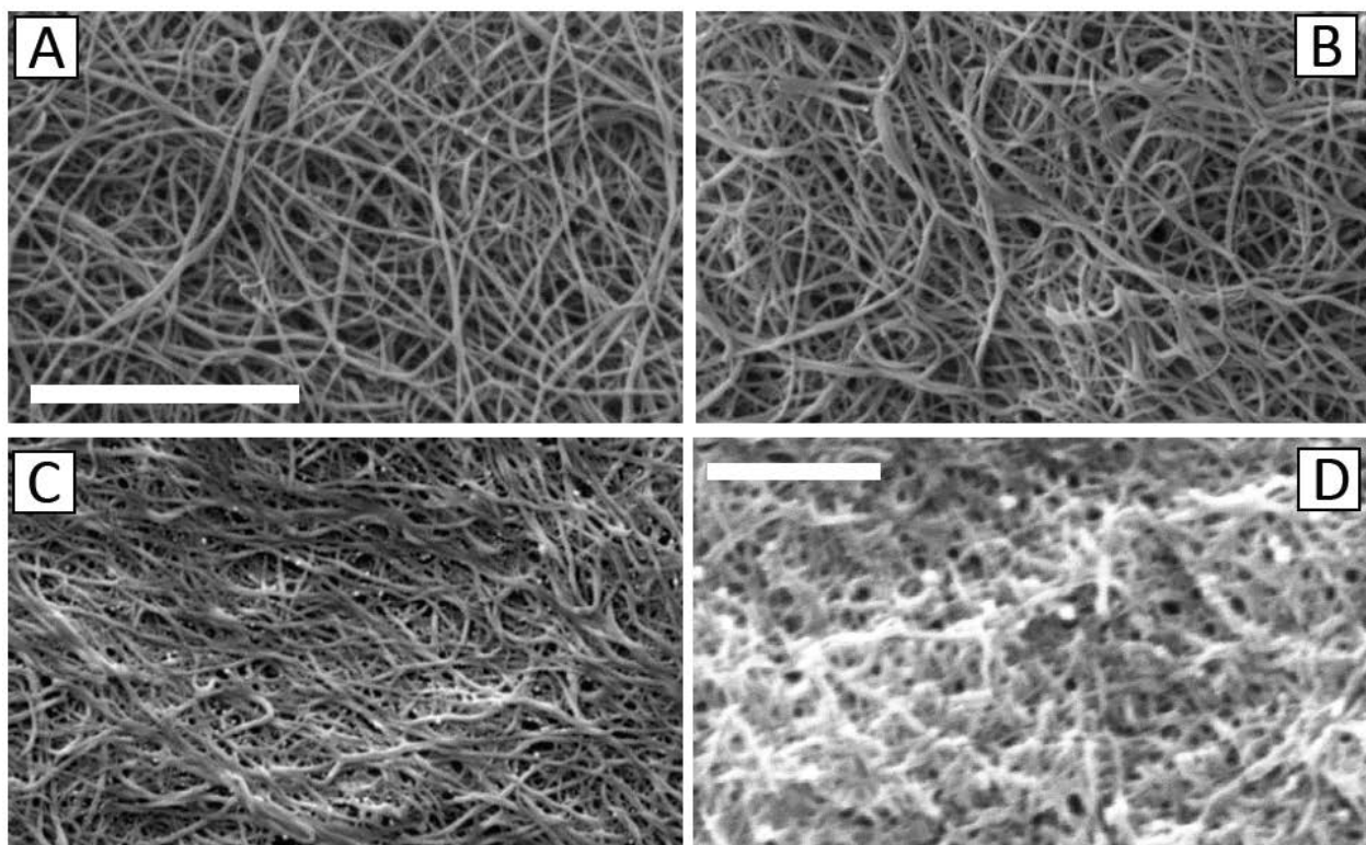
Figure S2. SEM images of fibrin networks. (A-C) Coarse fibrin networks polymerized at concentrations of 1, 3 and 7 mg/ml, respectively. Scale bar represents 5 \mu\text{m} for (A-C). (D) Fine fibrin network polymerized at a concentration of 1 mg/ml. Scale bar denotes 400 nm.
