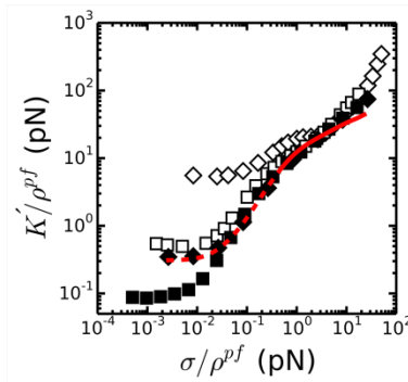
Fig. 6 Direct comparison of the high-stress (enthalpic) elastic response of bundled fibrin networks prepared under coarse conditions (open symbols) and fine fibrin networks (closed symbols). Data are shown for two protein concentrations: c_p = 0.5 (squares) and 3 (diamonds) mg/ml. The affine thermal model prediction for extensible wormlike chains for 3 mg/ml fine fibrin (red dashed line) is shown, where the enthalpic regime is indicated by the solid line.
