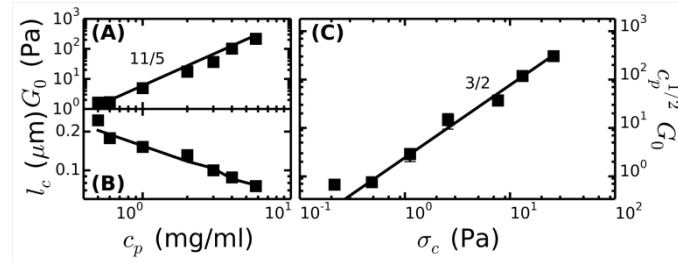
Fig 3 Comparison of rheology of fine fibrin networks (squares) with the affine thermal model for extensible wormlike chains (lines). (a) Plateau modulus, G_0 , as a function of fibrin concentration, c_p , compared with the predicted 11/5 power-law. (b) Cross-link distance, l_c , as a function of c_p compared with the theoretical prediction for l_c = l_e . (c) c_p^{1/2} G_0 shows a power-law dependence on \sigma_0 with an exponent of 3/2, consistent with the notion that G_0 and \sigma_0 are both governed by the entropic force–extension behavior of the filaments.
