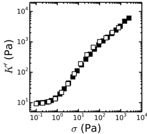
Figure S7. Nonlinear rheology of fine fibrin networks (2 mg/ml), in the presence (open squares) and absence (closed squares) of 200 \mu M D004, with 1% DMSO.
