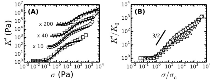
Fig. 2 Stress-stiffening response of fibrin networks prepared under fine network condition near the single protofibril limit ( N_p = 2 ), to an applied shear stress at different protein concentrations: c_p = 0.5 (squares), 1 (circles), 3 (triangles up) and 6 mg/ml (triangles down). In (A), the solid lines represent predictions of the affine thermal model for extensible chains. The K' values have been shifted vertically for clarity, as indicated. (B) Normalized stress-stiffening curves. Fine fibrin networks show clear evidence of fiber stretching at high strain, since the stiffening curve is weaker than the predicted 3/2-scaling (short solid line) expected for inextensible polymers.
