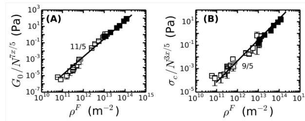
Fig. 5 The concentration dependences of (A) the plateau modulus G_0 and (B) the onset stress for stress-stiffening \sigma_0 of fibrin networks are both consistent with the semiflexible bundle model. This is demonstrated by rescaling G_0 and \sigma_0 for fine (solid squares) and coarse fibrin networks (open squares) by their dependence on N_p . The gray circle represents a fibrin network of 1 mg/ml prepared from gel-filtered fibrinogen, for which N_p = 366 . Coupling is assumed to be loose in case of fine fibrin ( \chi = 1 ) and tight for coarse fibrin ( \chi = 2 , see Fig. 4), and is found to be intermediate for the ultra-thick fibrin fibers ( N_p = 366 , \chi = 1.3 ).
