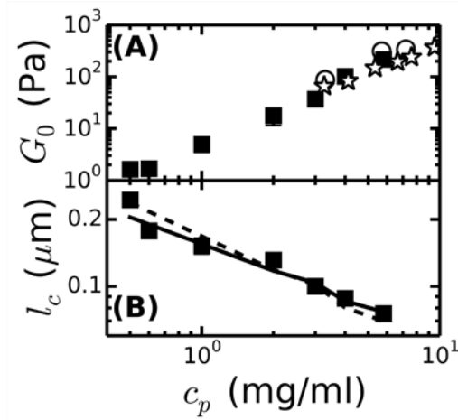
Figure S4. (A) The linear elastic modulus for fibrin clots polymerized under fine clot conditions, which show minimal bundling (black squares), compared with previous measurements (open circles: Ref. (1) and open stars: Ref. (2)). (B) Cross-link distance inferred by fitting the rheology data for fine clots to the affine model for wormlike chains to theoretical predictions according to l_c \sim l_e = l_p^{1/5} \rho^{-2/5} (solid line) or l_c \propto \rho^{-1/2} (dashed line), using a prefactor of 0.75 in both cases.
