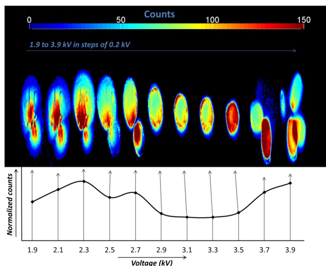
Figure 2. 3D representation of a z-stack of 2D contour maps showing the development of the ESI ion beam with the spray voltage increasing from 1.9 to 3.9 kV. Counts are represented on a normalized scale with the maximum at 2.3 kV for 294200 counts.
