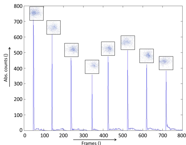
Figure 4. The total number of counts versus the frame number for a progressive wave chip experiment. The insets show the integrated signal per droplet application.
