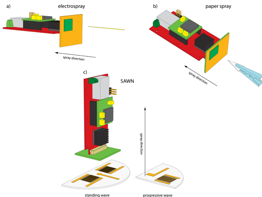
Figure 1. Illustration of the setups for (a) electrospray ionization, (b) paper spray ionization, and (c) two designs of surface acoustic wave nebulization, progressive wave and standing wave chip design.
