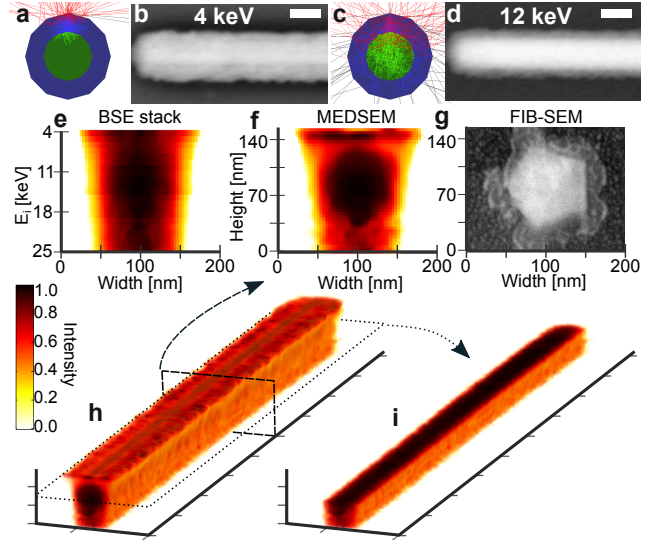
FIG. 2. Ag-Cu 2 O core-shell nanowire imaging. a , Diagram of primary electron (gray) and BSE (red) trajectories, and b , BSE SEM image demonstrating surface sensitivity at low acceleration energy, contrasted with c , d , showing high acceleration energy allowing the core of the nanowire to become visible. Scale bars are 100 nm. Cross-sectional slices of BSE image stack, e , before deconvolution, showing smearing between images from acceleration energies E_i , contrasted to the reconstruction, f , after deconvolution, showing the core clearly visible, and the nanowire extent realistically confined. The height is calibrated to the estimated nanowire total thickness. g , Comparison to FIB-SEM cross-sectional image. h , 3D reconstructions of the core-shell nanowire, with a surface slice through the X-Y plane in i , showing the Ag core (black) clearly visible throughout the imaged length. Tic marks are 200 nm in X and Y, 50 nm in Z. Pixel size is 3.4 nm.
