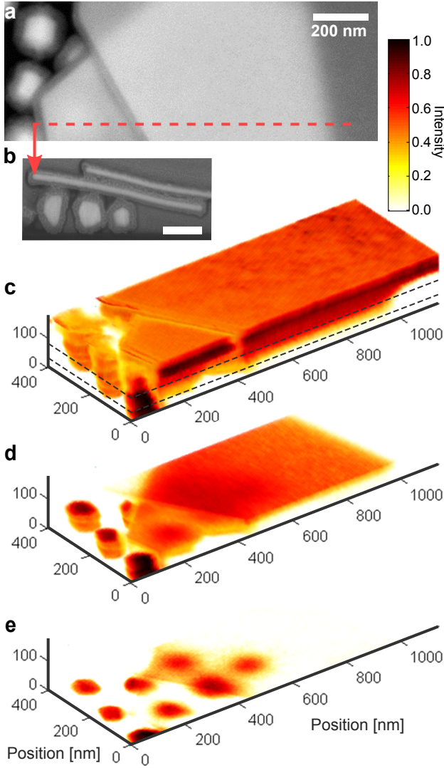
FIG. 4. a , BSE image of a double-layer Au-Cu 2 O sheet stack above Au-Cu 2 O core-shell nanoparticles. b , FIB-SEM cross section taken at the location indicated by the dashed line in a . c , 3D MEDSEM reconstruction of the nanostructure system. d , e , 3D MEDSEM reconstructions of surface slices through the X-Y plane (indicated in c ), displaying the variations of the imaged system with depth. Pixel size is 2.7 nm.
