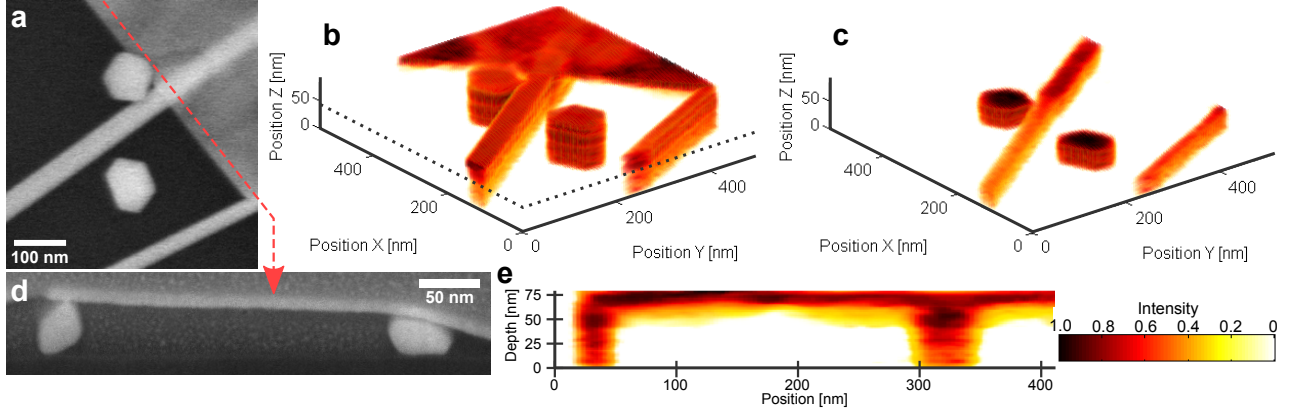
FIG. 3. a , BSE image of an Au sheet on top of two Au nanowires, with two Au nanoparticles adjacent. b , 3D MEDSEM reconstruction of the nanostructure system, as well as a surface slice (dotted line in b ) showing the region below the Au sheet in c . Cross-sectional views (taken through the dashed line in a ) using FIB-SEM in d , and the MEDSEM reconstruction in e , showing qualitative agreement. Pixel size is 4.5 nm.
