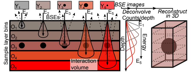
FIG. 1. Schematic of the MEDSEM process. A BSE image is composed of a superposition of virtual depth layers O_i in the measured sample. The mixing extends over deeper layers at higher primary beam energies, which corresponds to the increased depth of the BSE emission volume (left). This is represented by the counts per depth distributions (middle), which shows wider distribution curves at higher energies (increased redness). The deconvolved BSE images are then combined to form a 3D reconstruction of the nanomaterial (right).
