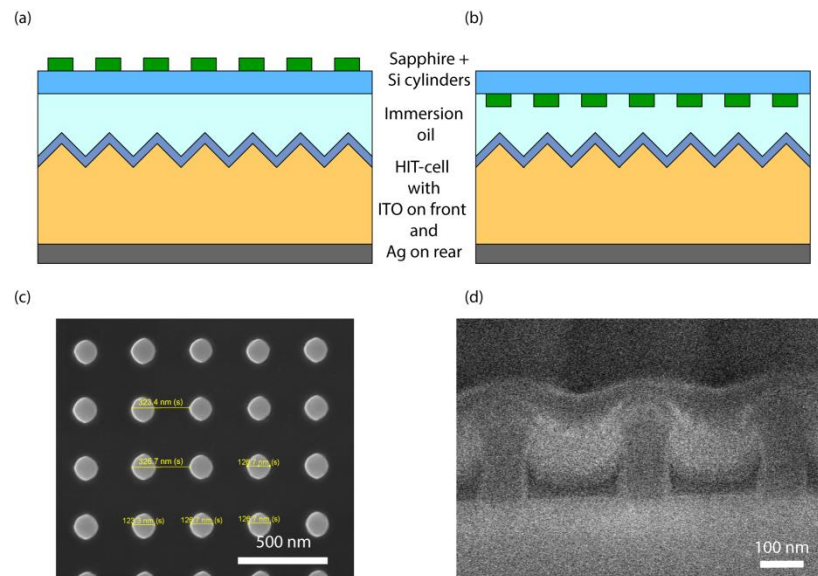
FIG. 1. Integrated Mie scattering designs for colored solar panels. (a,b) Schematic of silicon nanoscatterer arrays on top (a) and bottom (b) of a sapphire cover slide, integrated into a silicon heterojunction solar module using immersion oil. The sapphire slide and the immersion oil mimic commonly used module glass and EVA. (c) Top-view SEM image of a square array of silicon nanoscatterers on a sapphire cover slide, made by SCIL. (d) SEM image of a cross section of the silicon nanoscatterers on sapphire made using focused ion beam milling.
